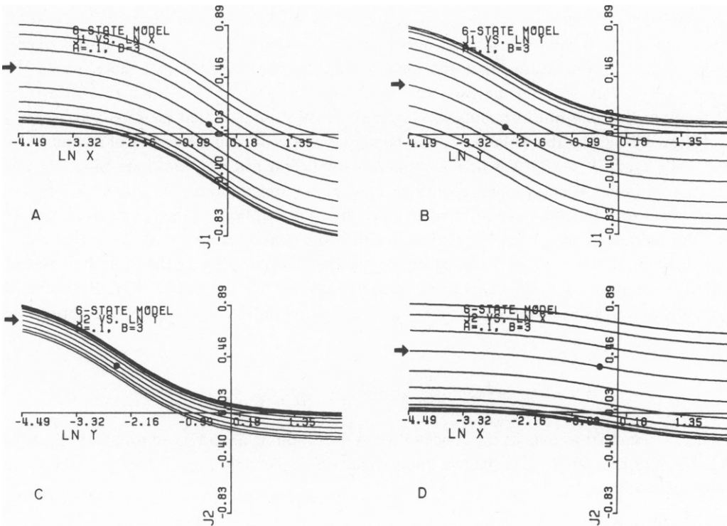
FIGURE 7 (A, B) Plots of Eq. 33a for a = 0.1 , b = 3.0 . In Fig. 7 A, J_1 is plotted as a function of \ln X for constant values of \ln Y = -4.49, -3.79, -3.09, -2.39, -1.68, -0.99, -0.29, 0.41, 1.14, 1.82 (starting from the upper curve). In Fig. 7 B J_1 is plotted as a function of \ln Y for the same constant values of \ln X listed above. (C, D) Plots of Eq. 33b for a = 0.1 , b = 3.0 . In Fig. 7 C J_2 is plotted as a function of \ln X for constant values of \ln Y (same as listed above.) In Fig. 7 D J_2 is plotted as a function of \ln Y for constant values of \ln X listed above. The dots represent inflection points.
