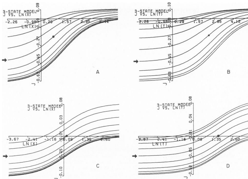
FIGURE 4 (A, B) Plots of Eq. 26 for the rate constants a = 1 , b = 3 , c = 1 , d = 5 , e = 1 , \mathcal{F} = 0.1 . (A) J plotted as a function of \ln x_1 = \ln X for constant values of \ln x_2 = \ln Y . Starting from the upper curve \ln Y = 4.63, 3.87, 3.11, 2.34, 1.57, 0.81, 0.04, -0.73, -1.49, -2.26 . The dot denotes the two-dimensional inflection point at \ln X = 0.81 , \ln Y = 2.34 . (B) J plotted as a function of \ln x_2 = \ln Y for constant values of \ln X (same as above) (C, D) Plots of Eq. (26) for the rate constants a = 1 , b = 0.114 , c = 1 , d = 5 , e = 1 , \mathcal{F} = 0.1 . In this case \ln Y (C) or \ln X (D) has the constant values starting from the upper curve of 3.11, 2.35, 1.63, 0.85, 0.10, -0.66, -1.41, -2.16, -2.91, -3.66 . The dot marks the two-dimensional inflection point at \ln X = 0.10 and \ln Y = 1.63 . In this case the rate constants were chosen so that X^0, Y^0 coincides with equilibrium.
